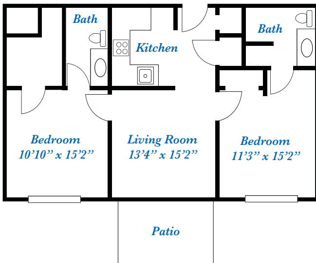
Two Bedroom Deluxe 897 sq. ft.
